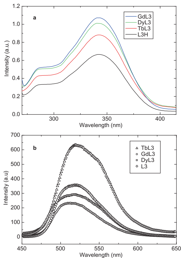
Figure 14. (a) UV-visible optical absorption spectra of ligand L 3 H and complexes GdL 3 , DyL 3 and TbL 3 recorded in chloroform at the same concentration ( c = 1 \times 10^{-5} mol L -1 ); and (b) emission spectrum of ligand and complexes recorded in chloroform at the same concentration ( c = 1 \times 10^{-5} mol L -1 ).
