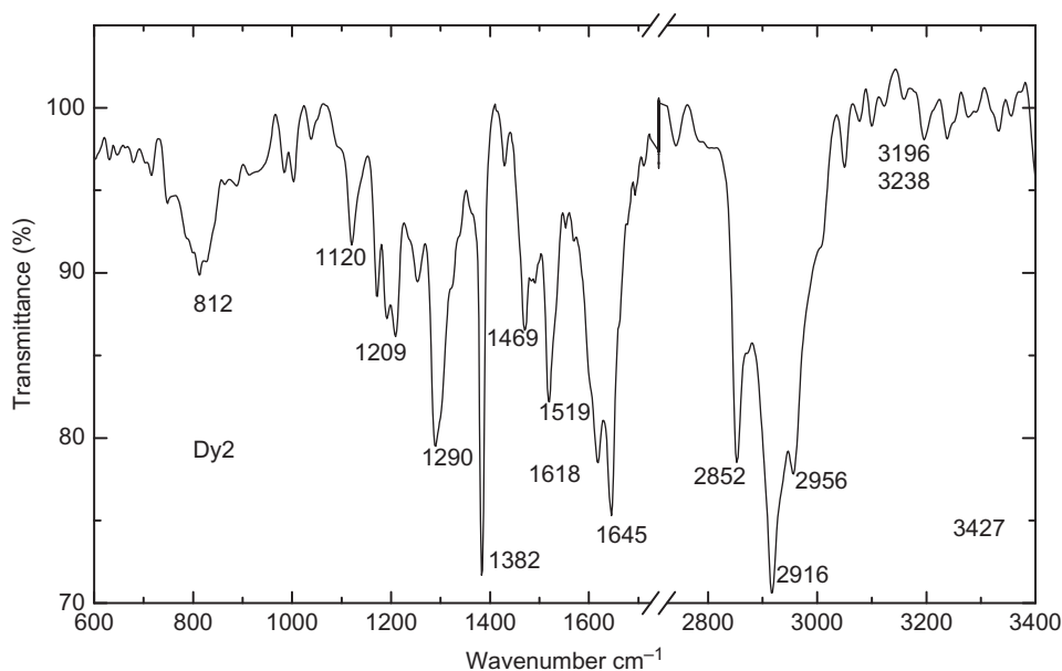
Figure 4. Representative FTIR spectrum of \text{Dy}_2 .
