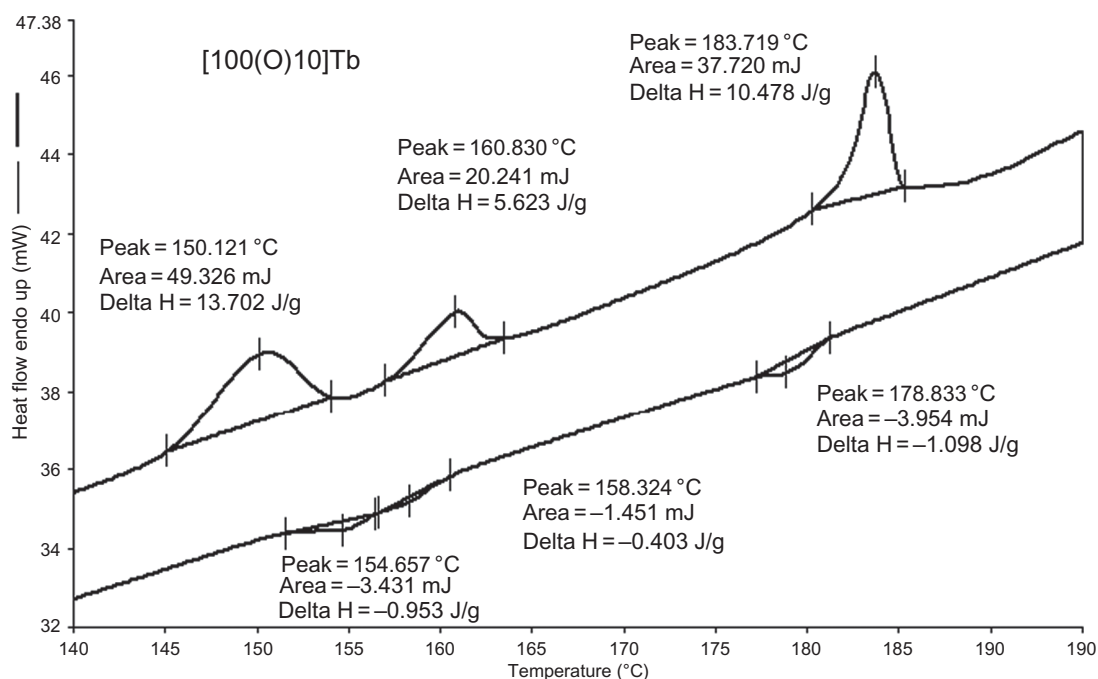
Figure 8. DSC spectrum of Tb2.
